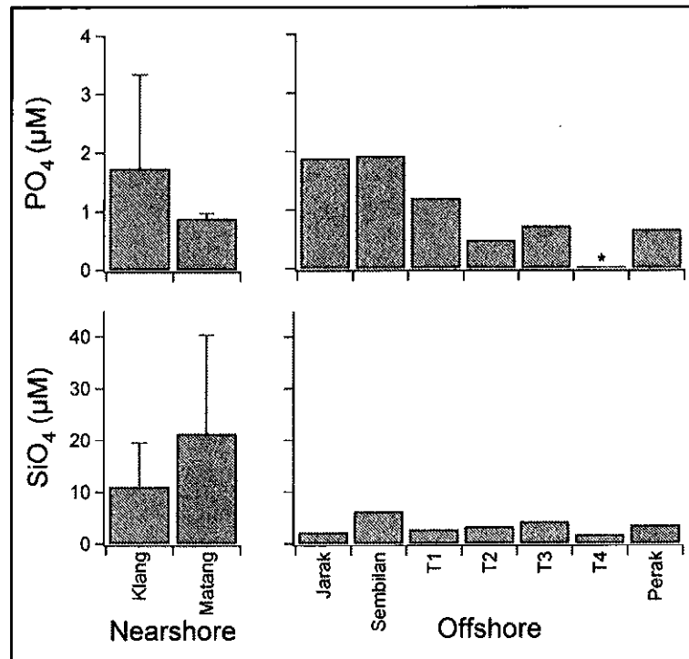
Figure 4. Average phosphorus (PO 4 , μM) and silicate (SiO 4 , μM) concentrations nearshore and offshore. Error bars (± Standard Deviation) for nearshore stations are also shown. * - data not available.
