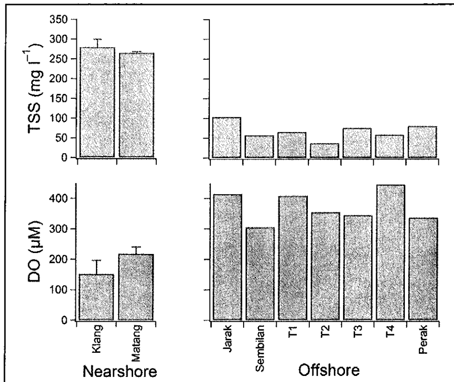
Figure 2. Average total suspended solids (TSS, mg l -1 ) and dissolved oxygen (DO, μM) nearshore and offshore. Error bars ( \pm Standard Deviation) for nearshore stations are also shown.
