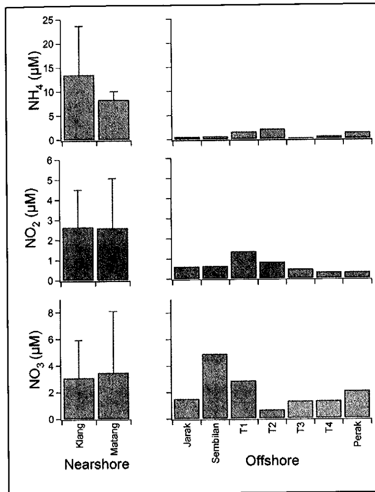
Figure 3. Average ammonium (NH 4 , µM), nitrite (NO 2 , µM) and nitrate (NO 3 , µM) concentrations nearshore and offshore. Error bars (± Standard Deviation) for nearshore stations are also shown.
